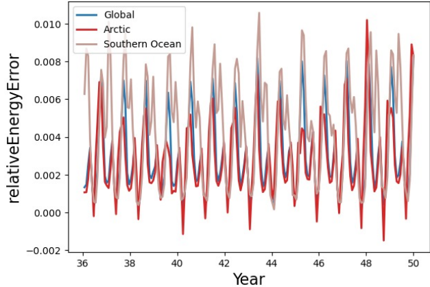
Feature relativeEnergyError (Sea ice)
