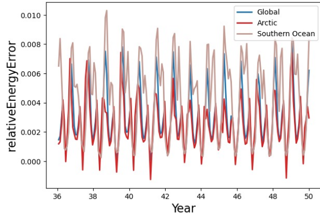
Control relativeEnergyError (Sea ice)
