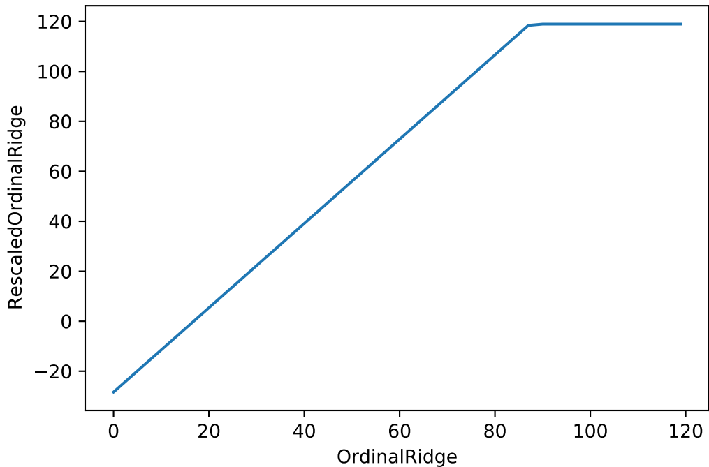
Predictions of Ordinal Ridge vs Rescaled Ordinal Ridge
