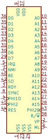
U1 W65C025xxPLx-14
