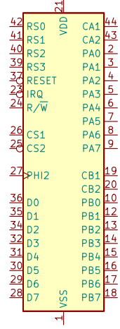
U7 W65C225xxPLx-14
