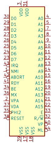
U5 W65C8165xxPQx-14
