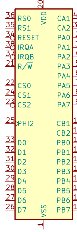
U7 W65C215xxPx-14
