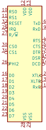
U7 W65C51NxxPQx-14
