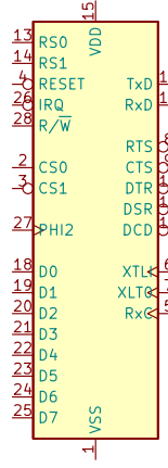
U7 W65C51NxxPx-14
