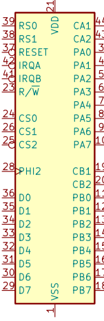
U7 W65C215xxPLx-14
