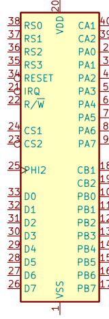
U7 W65C225xxPx-14
