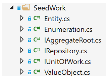
Figure 7-12. A sample set of domain model "seedwork" base classes and interfaces
