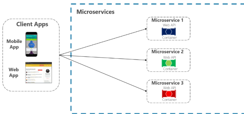
Figure 4-12. Using a direct client-to-microservice communication architecture
