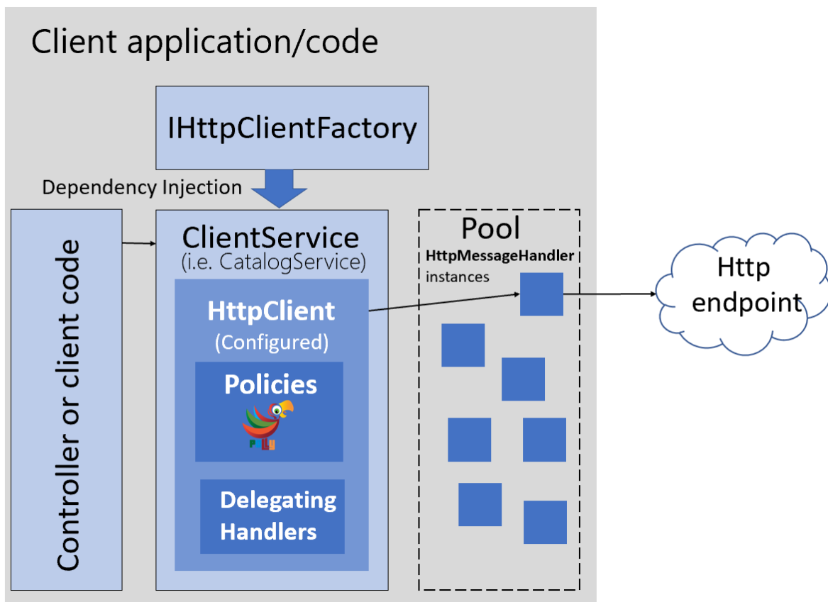
Figure 8-4. Using IHttpConnectionFactory with Typed Client classes.
