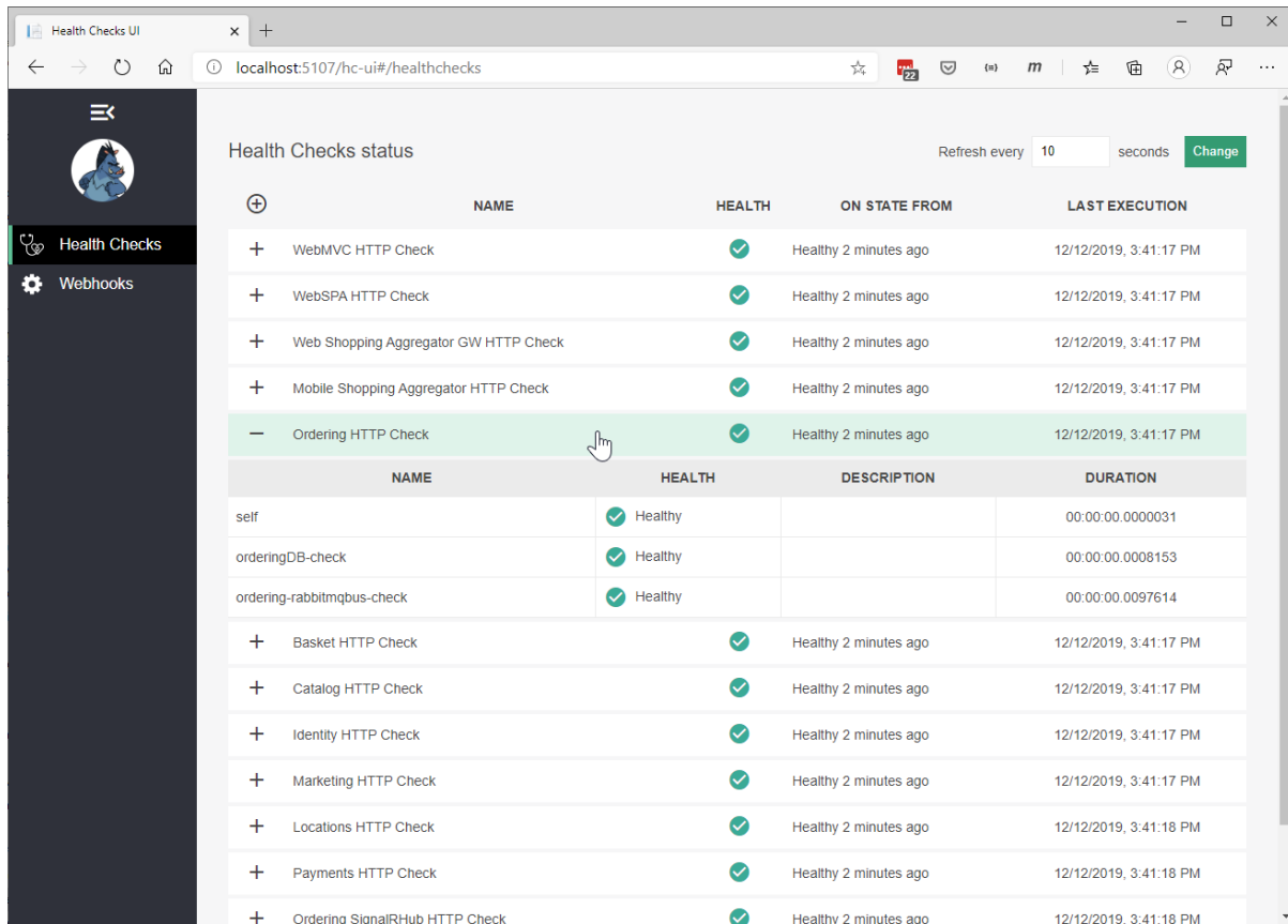
Figure 8-9. Sample health check report in eShopOnContainers
