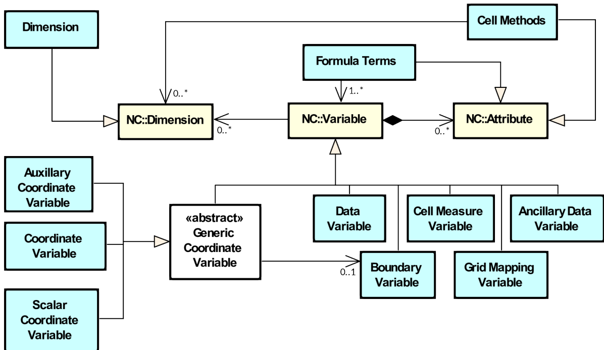
Figure 4. The relationships between CF-netCDF elements and their corresponding netCDF variables, dimensions and attributes (defined in figure 3 and identified here with the "NC" prefix). It is useful to define an abstract generic coordinate variable that can be used to refer to coordinates when their type (coordinate, auxiliary or scalar coordinate variable) is not an issue. The CF convention details the mechanisms which are used in the netCDF file to express the relationships among the CF-netCDF elements, but these are not shown.
