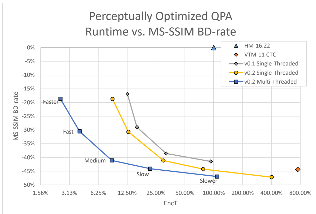
Figure 2: MS-SSIM BD-rate gain and encoder runtime in comparison to HM-16.22 for VTM and VVenC with QPA enabled. VVenC results are given for the 5 preset options: faster, fast, medium, slow and slower. Lower MS-SSIM BD-rate values mean a better compression for the same quality in terms of MS-SSIM.
