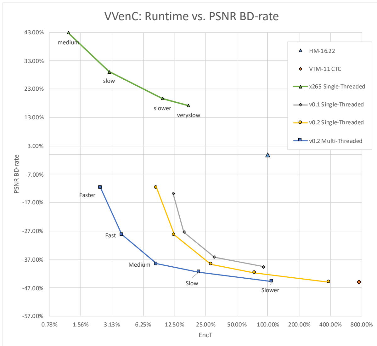
Figure 1: PSNR BD-rate gain and relative encoder runtime in comparison to HM-16.22 for VVenC, VTM and x265. Results are given for the 5 preset options: faster, fast, medium, slow and slower. Lower PSNR BD-rate values mean a better compression for the same objective quality in terms of PSNR.
