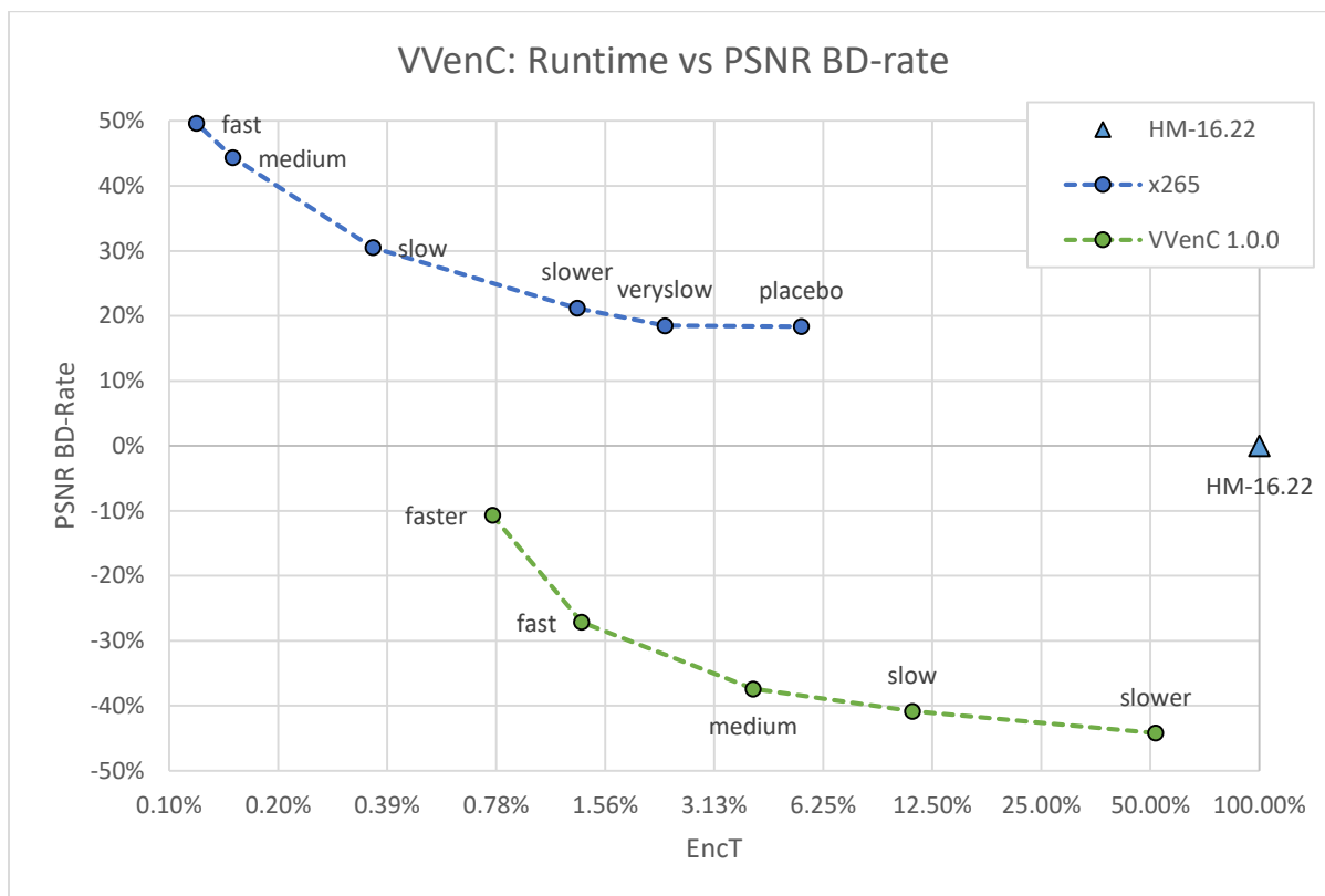
Figure 2: PSNR BD-rate gain and relative encoder runtime in comparison to HM-16.22 for VVenC and x265 running with 8 threads. Lower PSNR BD-rate values mean a better compression for the same objective quality in terms of PSNR.
