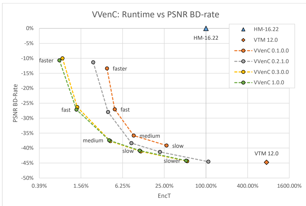
Figure 1: PSNR BD-rate gain and relative encoder runtime in comparison to HM-16.22 for VVenC and VTM. Results are given for the 5 preset options: faster, fast, medium, slow and slower. Lower PSNR BD-rate values mean a better compression for the same objective quality in terms of PSNR.
