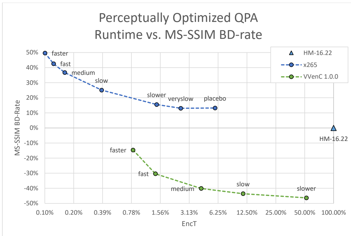
Figure 4: MS-SSIM BD-rate gain and encoder runtime in comparison to HM-16.22 for VVenC with QPA enabled and x265 with --tune=ssim. Lower MS-SSIM BD-rate values mean a better compression for the same quality in terms of MS-SSIM.
