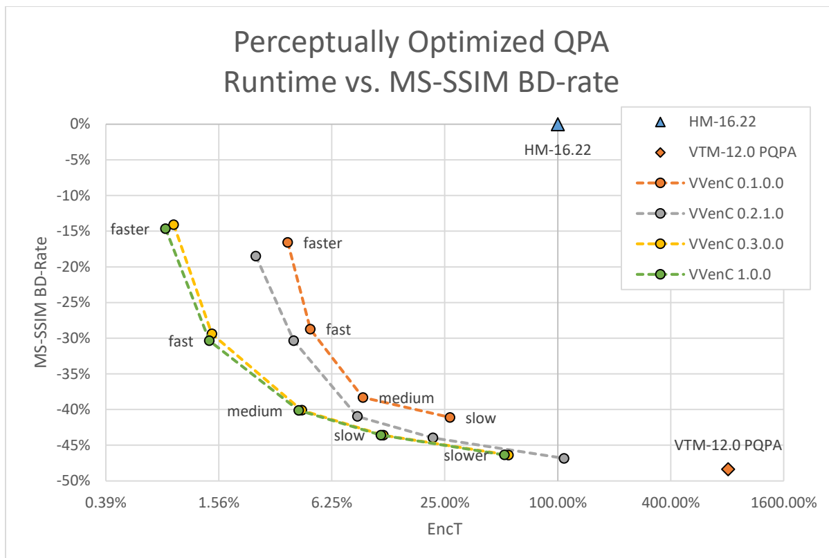
Figure 3: MS-SSIM BD-rate gain and encoder runtime in comparison to HM-16.22 for VTM and VVenC with perceptually optimized quantization parameter adaptation enabled. VVenC results are given for the 5 preset options: faster, fast, medium, slow and slower. Lower MS-SSIM BD-rate values mean a better compression for the same quality in terms of MS-SSIM.
