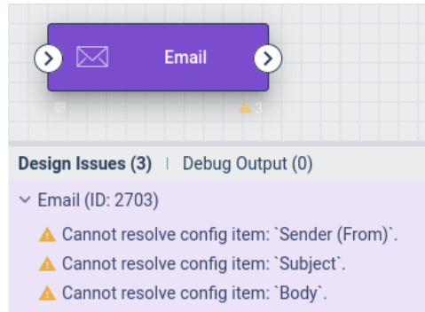
Figure 8.13: Parse errors.
