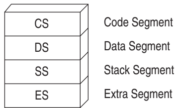
Figure 1.3 Registers for 8088–80286 Processors
