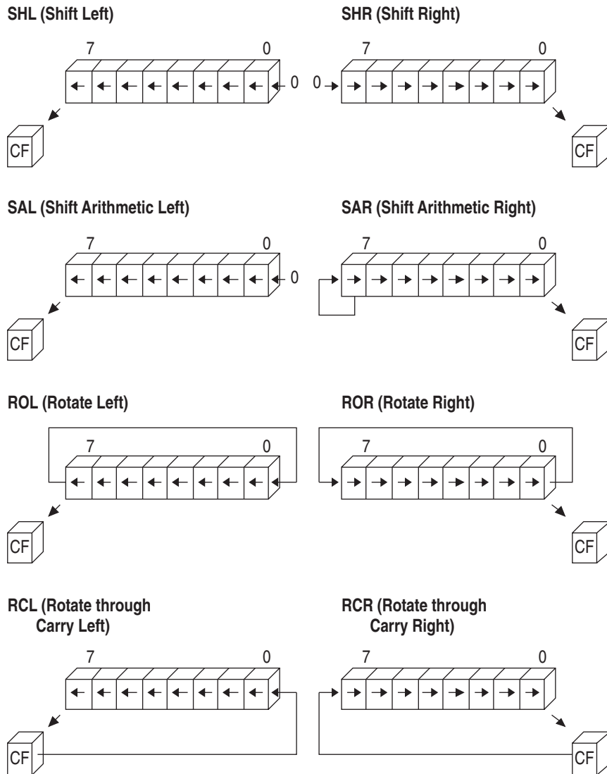
Figure 4.2 Shifts and Rotates
