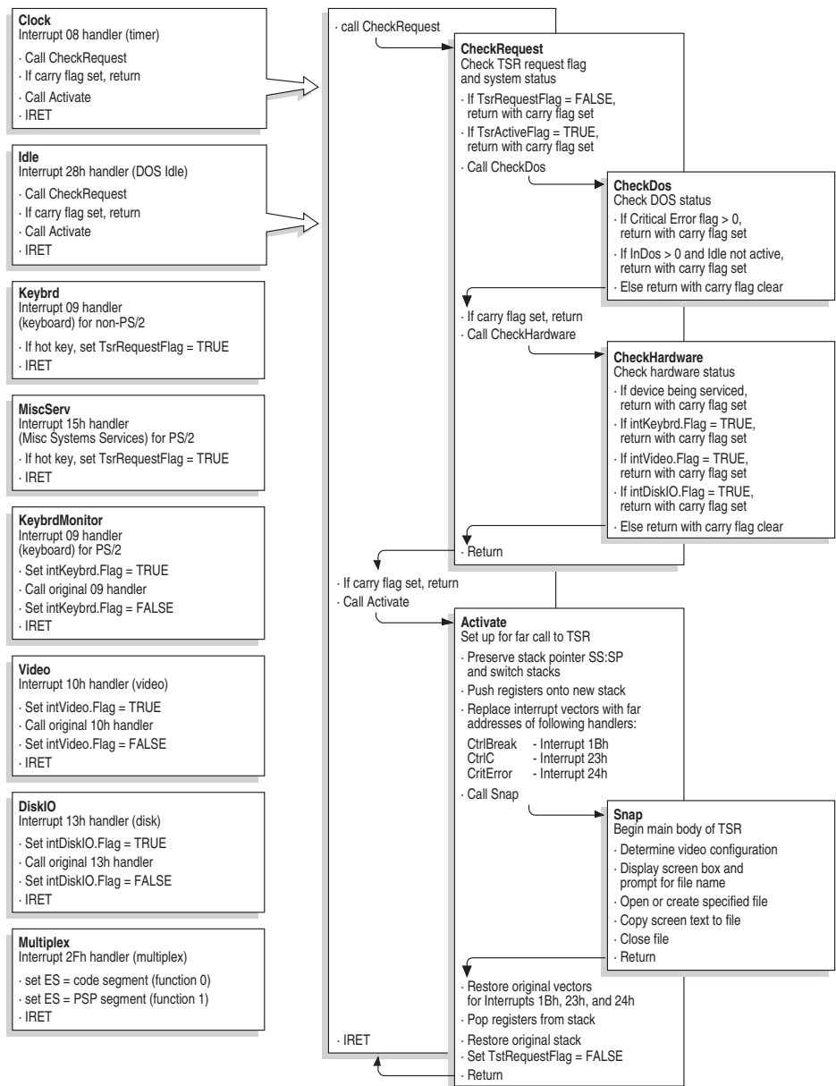
Figure 11.3 Flowchart for SNAP.EXE: Resident Phase
