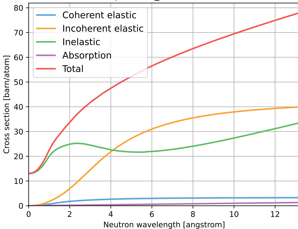
AcrylicGlass_C5O2H8.ncmat
