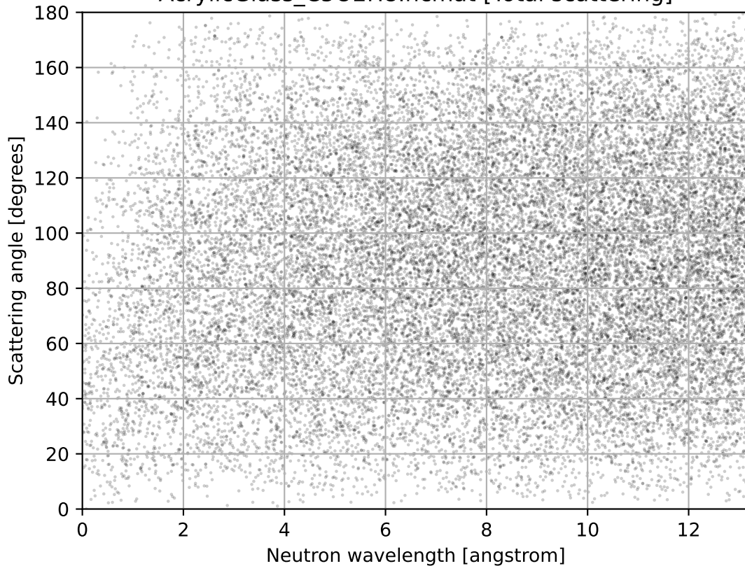
AcrylicGlass_C5O2H8.ncmat [Total scattering]
