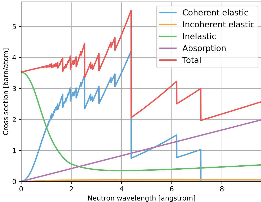
BaF2_sg225_BariumFluoride.ncmat
