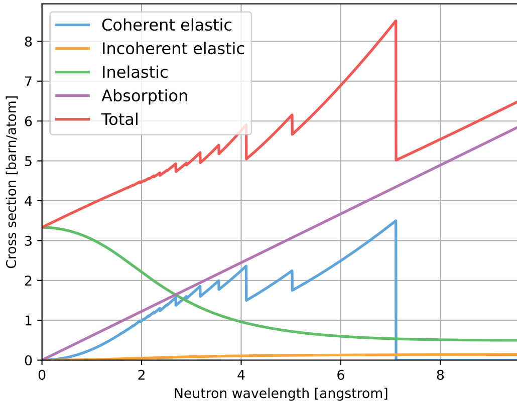
Ba_sg229.ncmat
