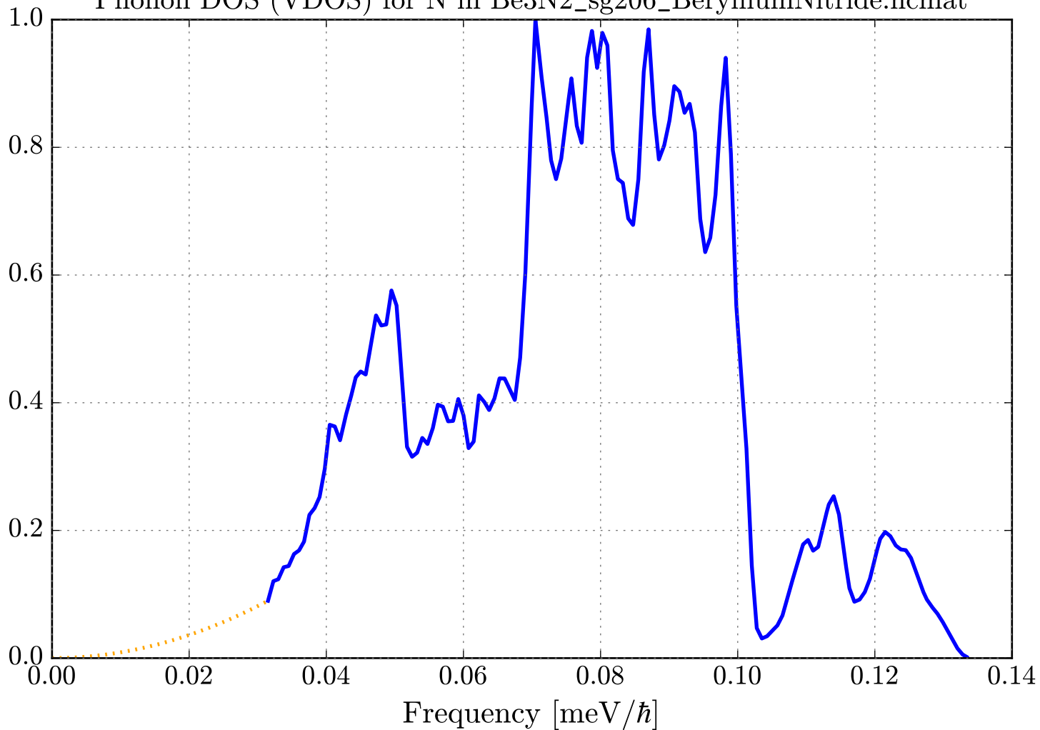
Phonon DOS (VDOS) for N in Be3N2_sg206_BerylliumNitride.ncmat
