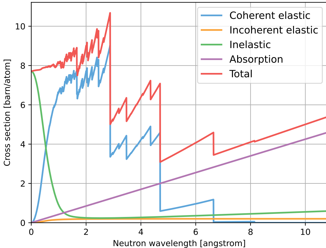
Be3N2_sg206_BerylliumNitride.ncmat
