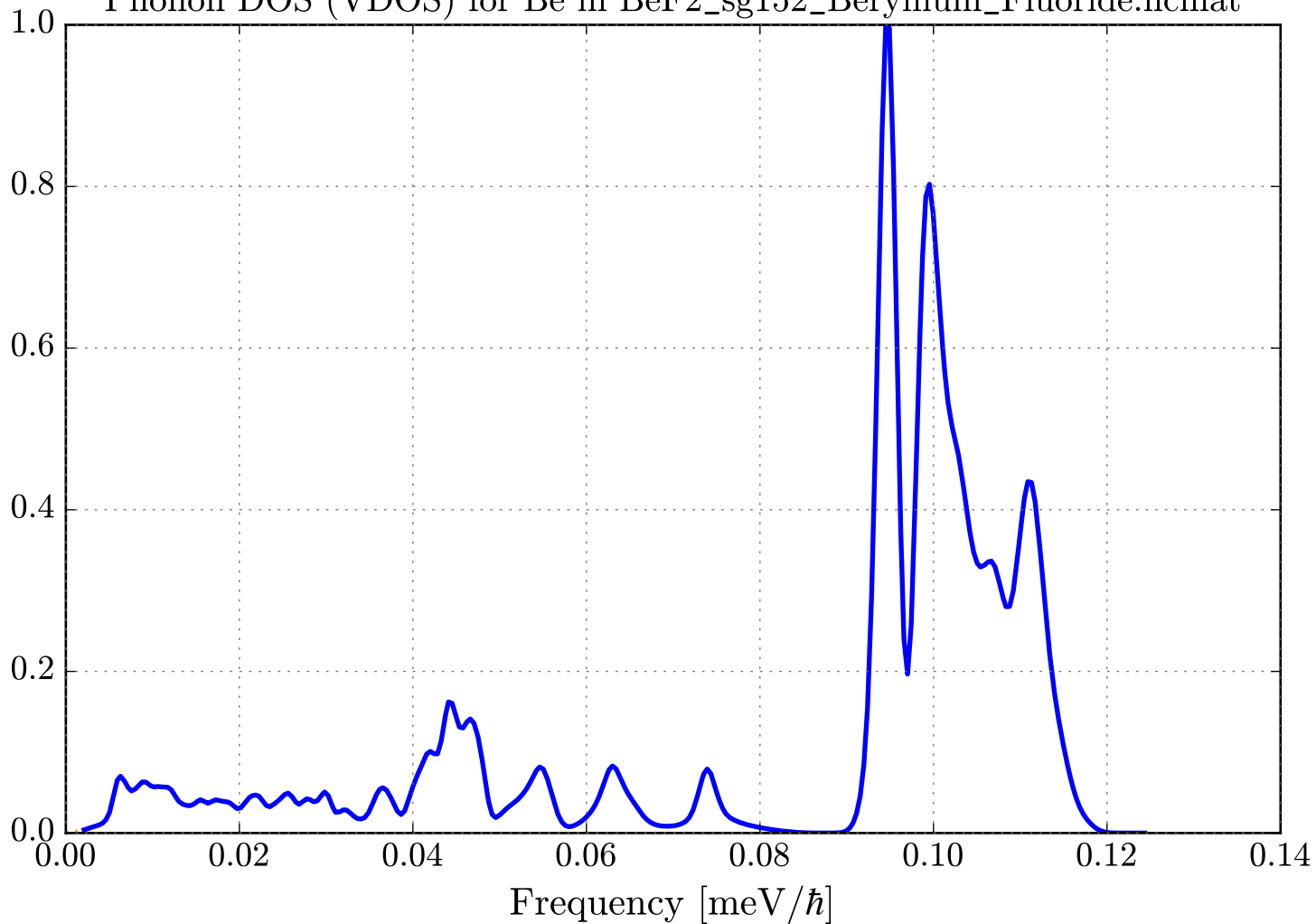
Phonon DOS (VDOS) for Be in BeF2_sg152_Beryllium_Fluoride.ncmat
