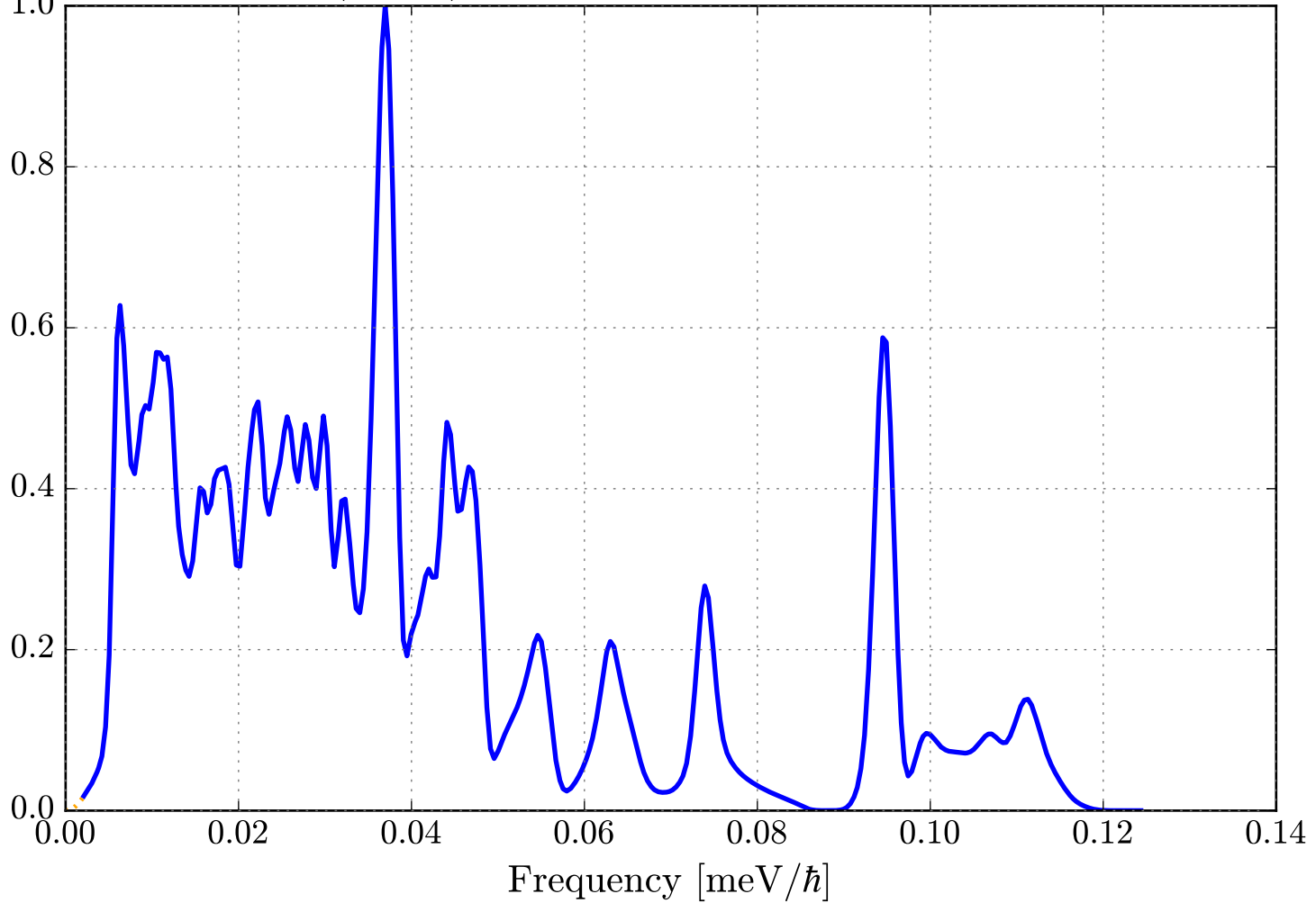
Phonon DOS (VDOS) for F in BeF2_sg152_Beryllium_Fluoride.ncmat
