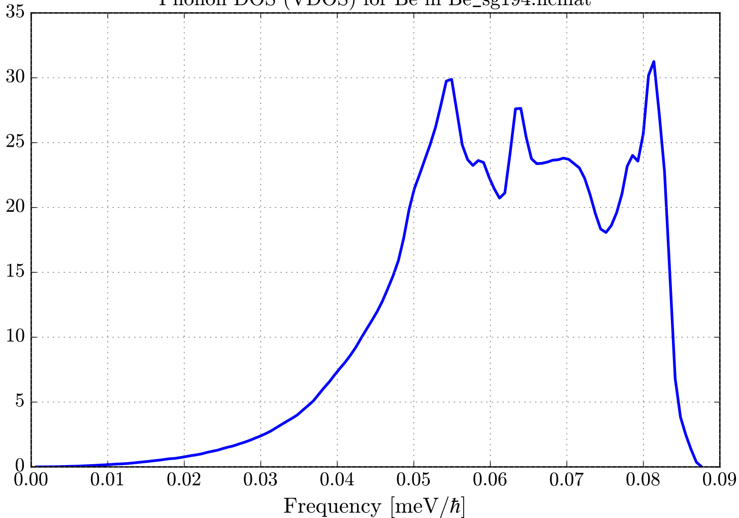
Phonon DOS (VDOS) for Be in Be_sg194.ncmat
