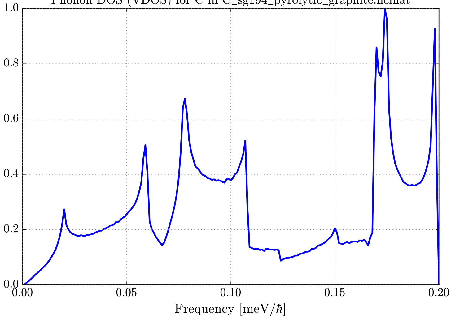
Phonon DOS (VDOS) for C in C_sg194_pyrolytic_graphite.ncmat
