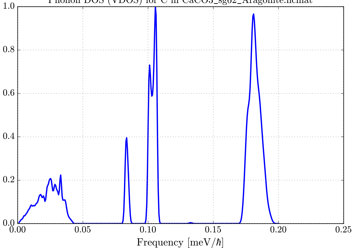
Phonon DOS (VDOS) for C in CaCO 3 _sg62_Aragonite.ncmat
