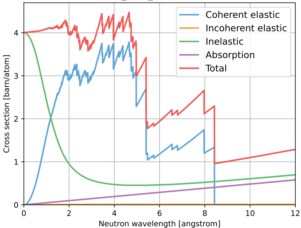
CaCO3_sg62_Aragonite.ncmat
