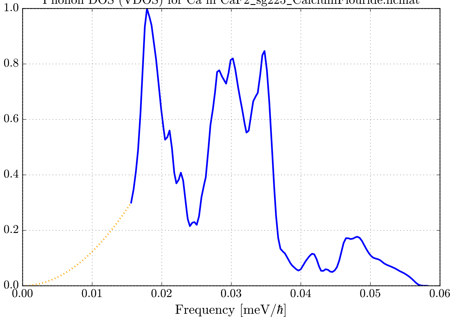
Phonon DOS (VDOS) for Ca in CaF2_sg225_CalciumFlouride.ncmat
