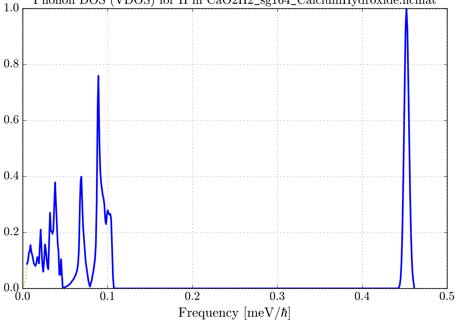
Phonon DOS (VDOS) for H in CaO2H2_sg164_CalciumHydroxide.ncmat
