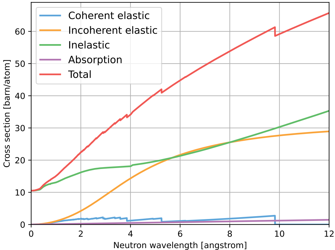
CaO2H2_sg164_CalciumHydroxide.ncmat
