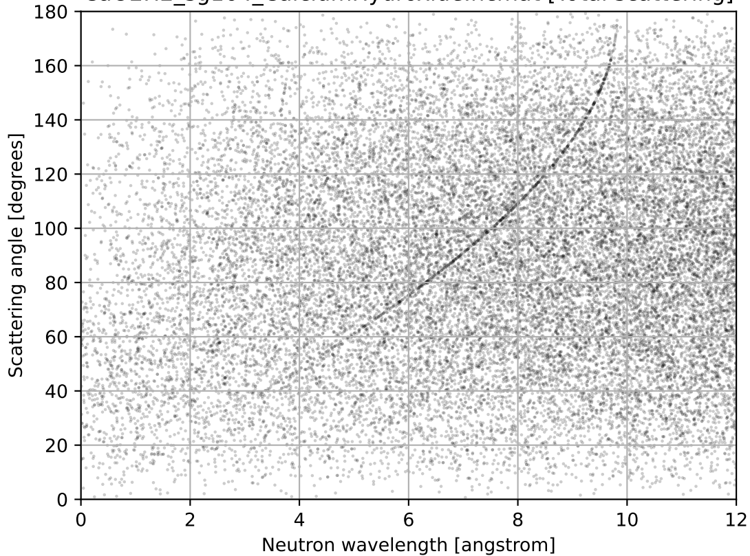
CaO2H2_sg164_CalciumHydroxide.ncmat [Total scattering]
