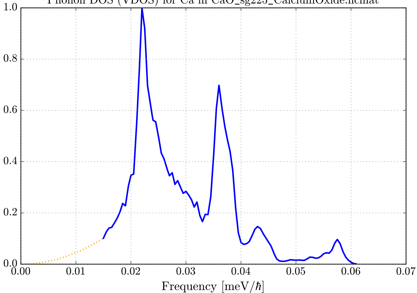
Phonon DOS (VDOS) for Ca in CaO_sg225_CalciumOxide.ncmat
