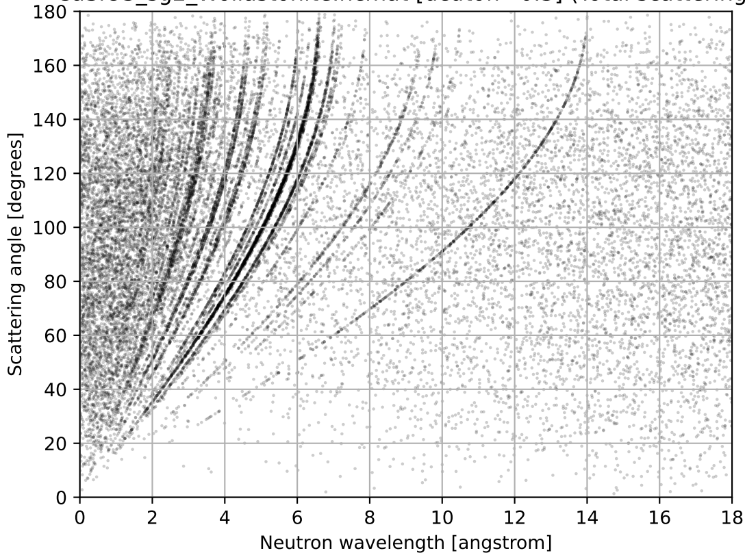
CaSiO3_sg2_Wollastonite.ncmat [dcutoff=0.3] (Total scattering)
