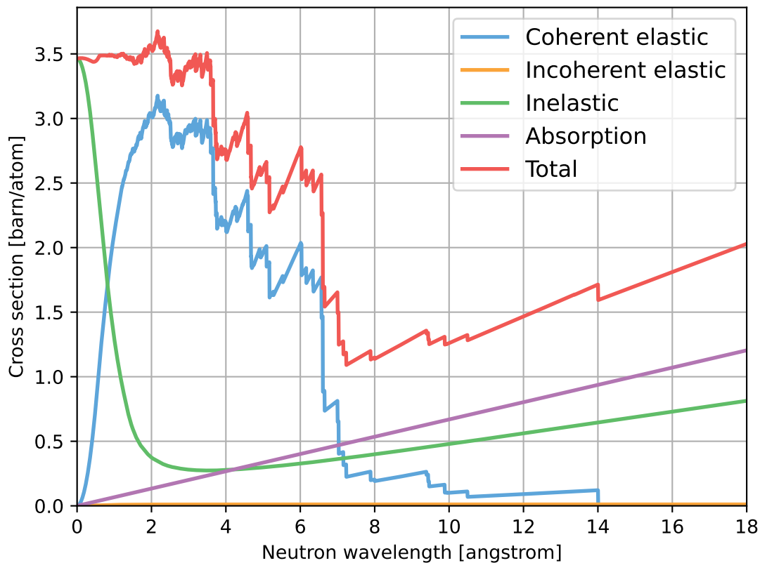
CaSiO3_sg2_Wollastonite.ncmat [dcutoff=0.3]
