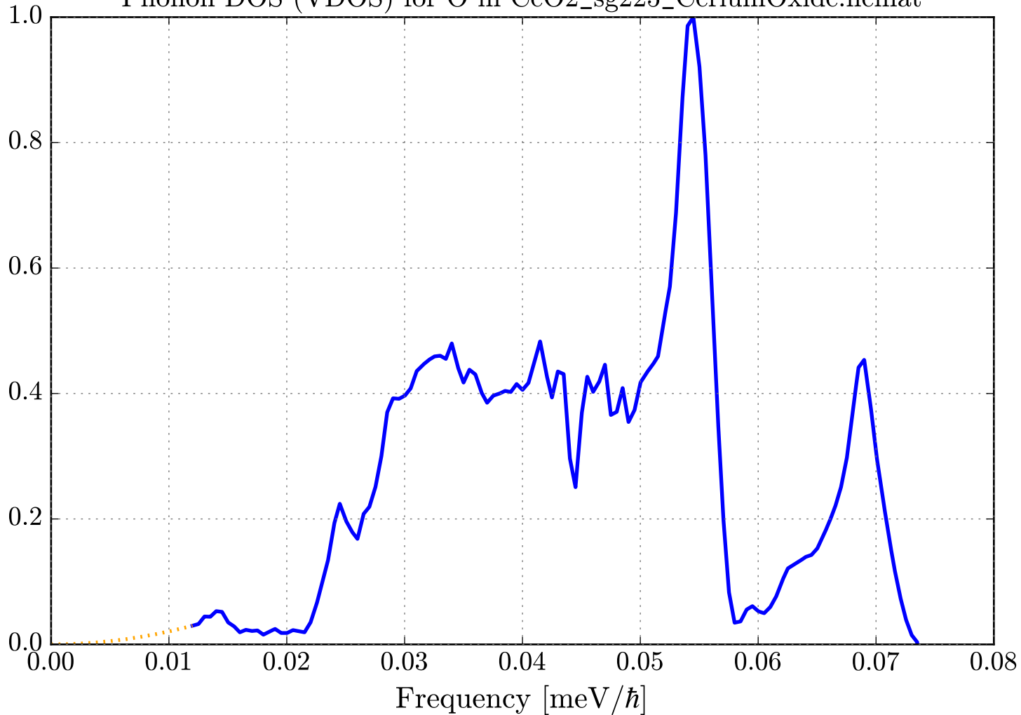
Phonon DOS (VDOS) for O in CeO2_sg225_CeriumOxide.ncmat
