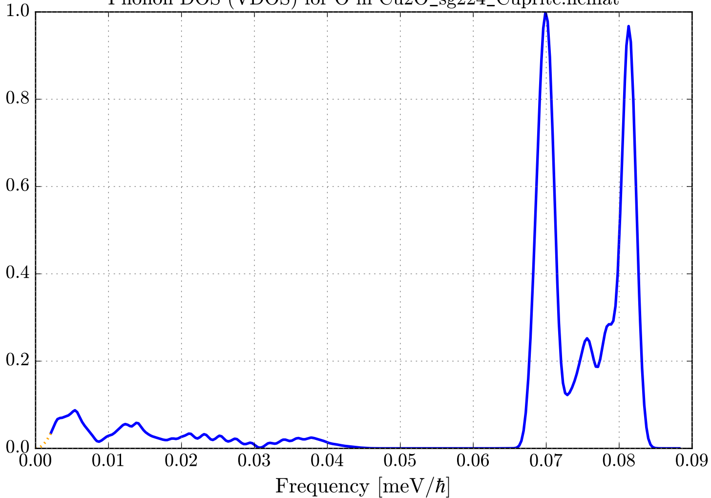
Phonon DOS (VDOS) for O in Cu 2 O_sg224_Cuprite.ncmat
