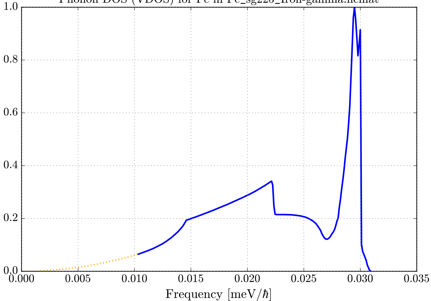
Phonon DOS (VDOS) for Fe in Fe_sg225_Iron-gamma.ncmat
