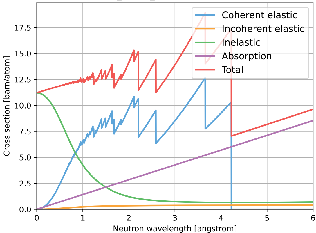
Fe_sg225_Iron-gamma.ncmat
