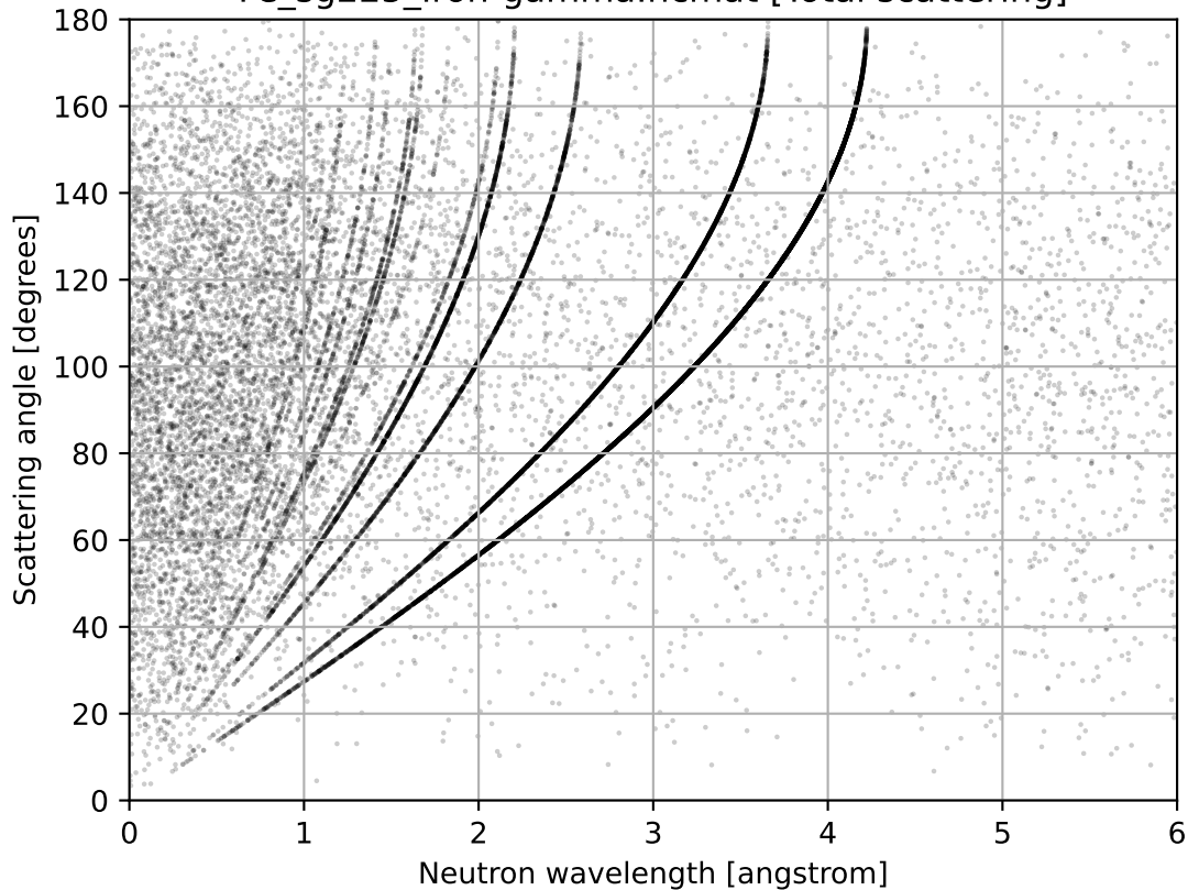
Fe_sg225_Iron-gamma.ncmat [Total scattering]
