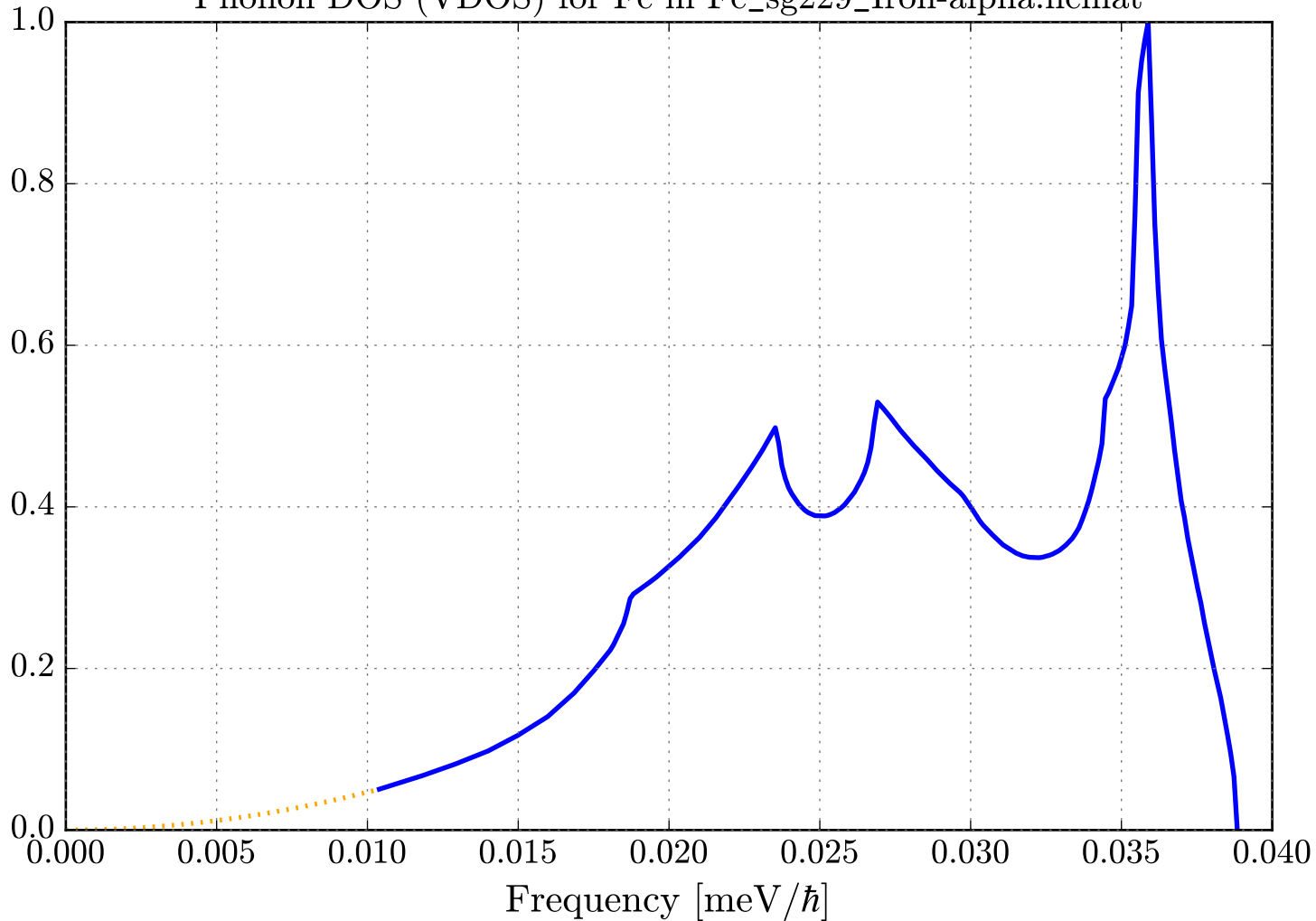
Phonon DOS (VDOS) for Fe in Fe_sg229_Iron-alpha.ncmat
