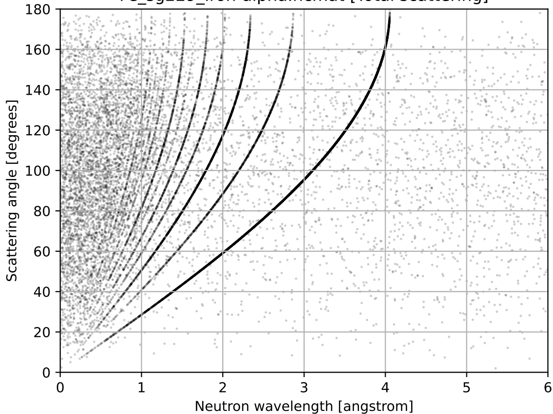
Fe_sg229_Iron-alpha.ncmat [Total scattering]
