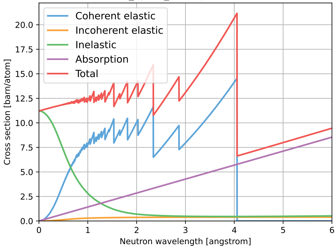
Fe_sg229_Iron-alpha.ncmat
