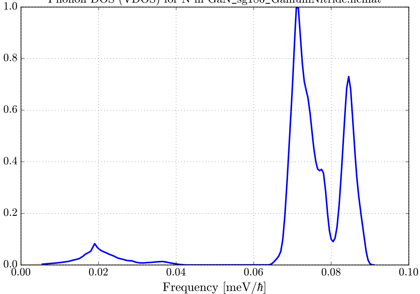
Phonon DOS (VDOS) for N in GaN_sg186_GalliumNitride.ncmat
