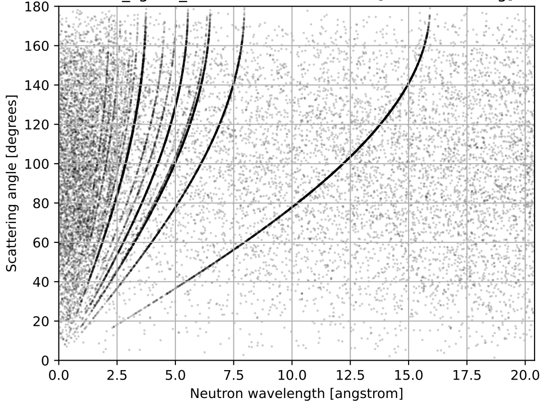
GaSe_sg194_GalliumSelenide.ncmat [Total scattering]
