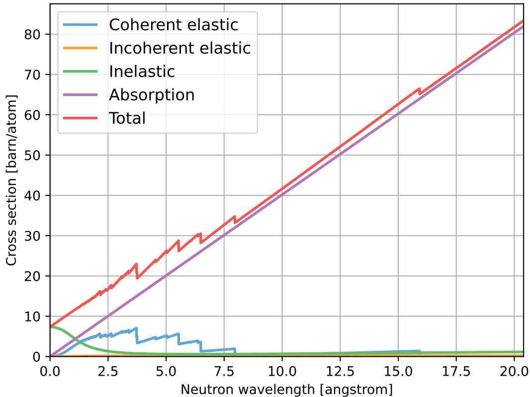
GaSe_sg194_GalliumSelenide.ncmat
