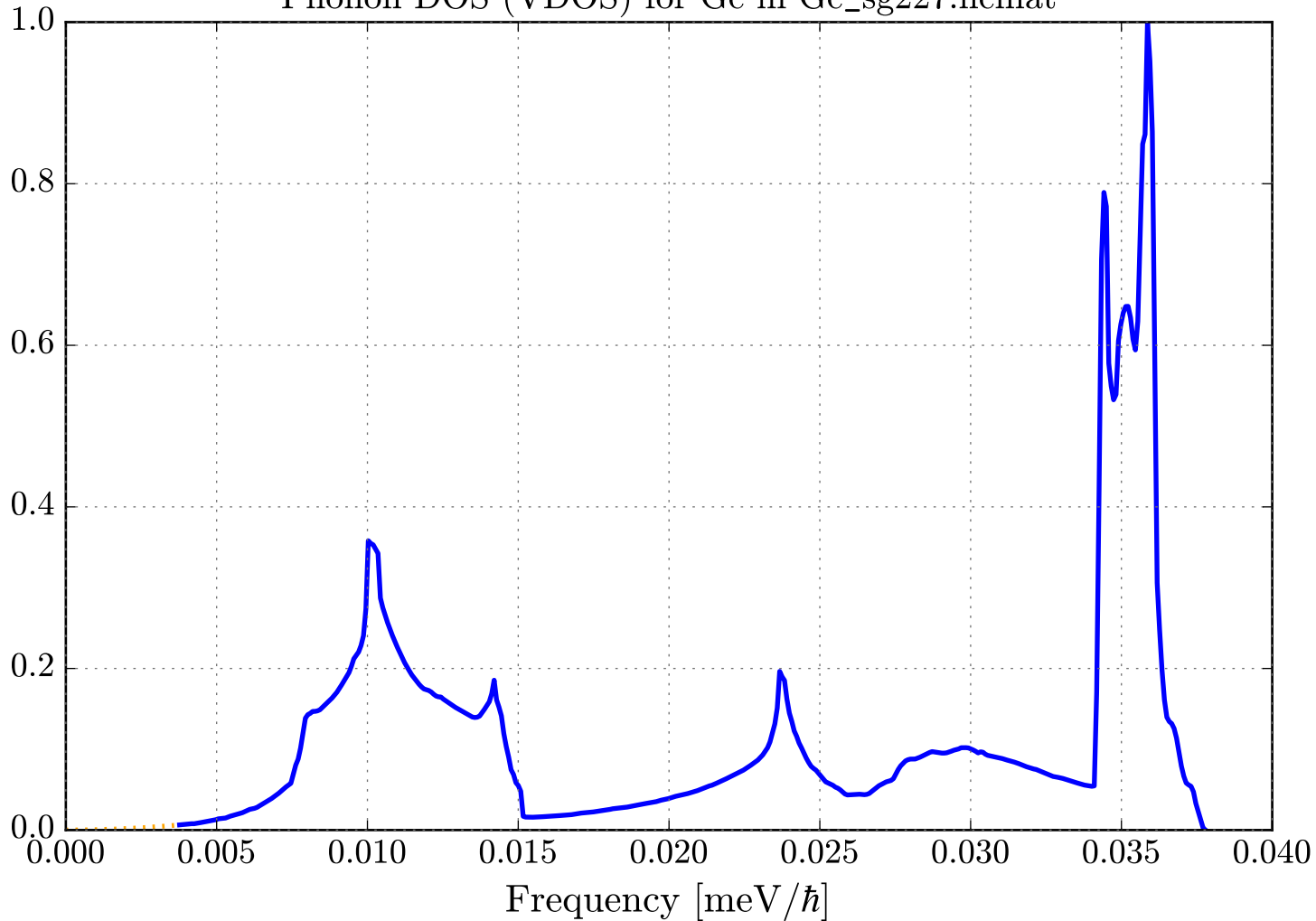
Phonon DOS (VDOS) for Ge in Ge_sg227.ncmat
