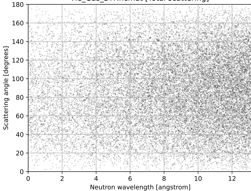
He_Gas_STP.ncmat [Total scattering]
