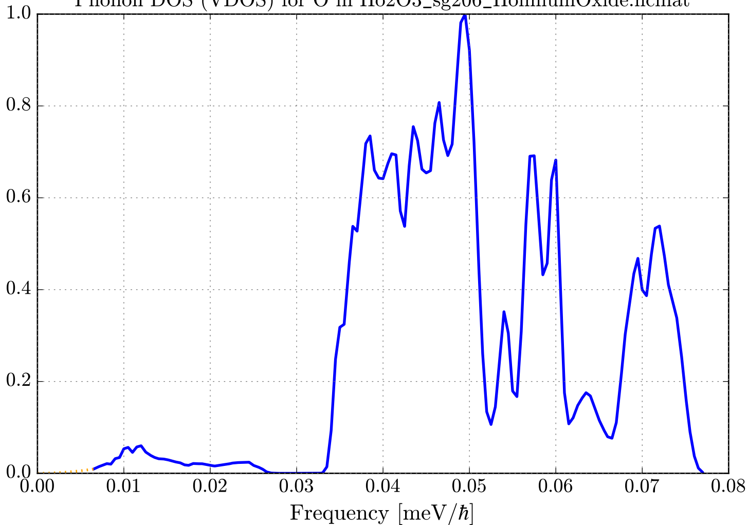
Phonon DOS (VDOS) for O in Ho2O3_sg206_HolmiumOxide.ncmat
