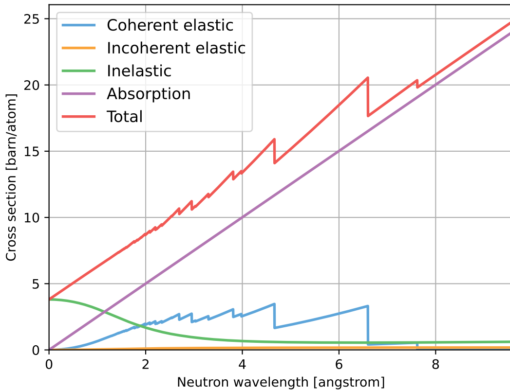
KBr_sg225_PotassiumBromide.ncmat
