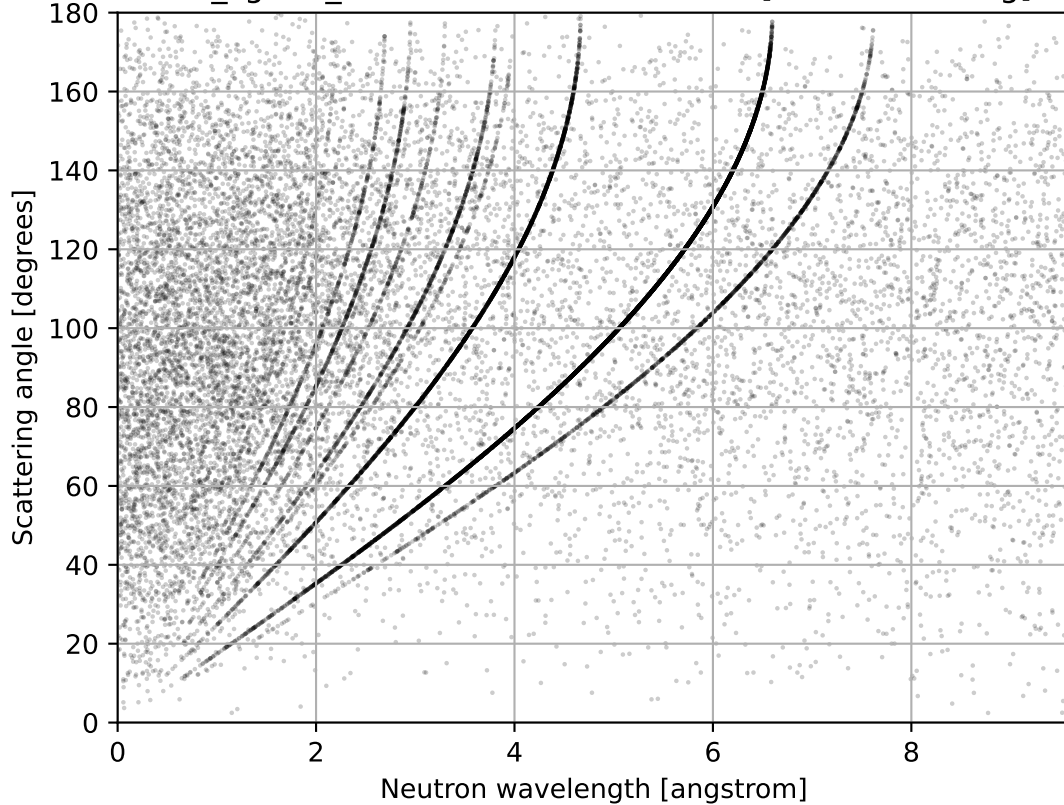
KBr_sg225_PotassiumBromide.ncmat [Total scattering]
