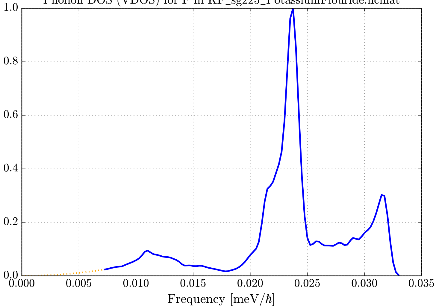
Phonon DOS (VDOS) for F in KF_sg225_PotassiumFlouride.ncmat
