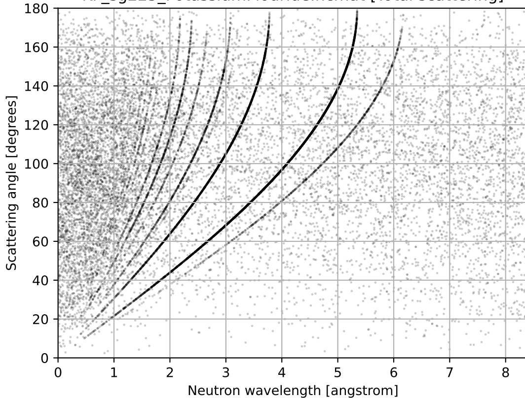
KF_sg225_PotassiumFlouride.ncmat [Total scattering]
