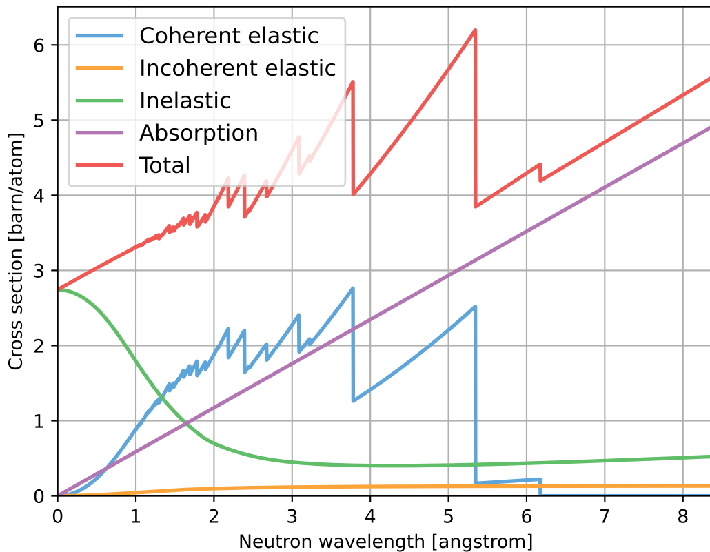
KF_sg225_PotassiumFlouride.ncmat
