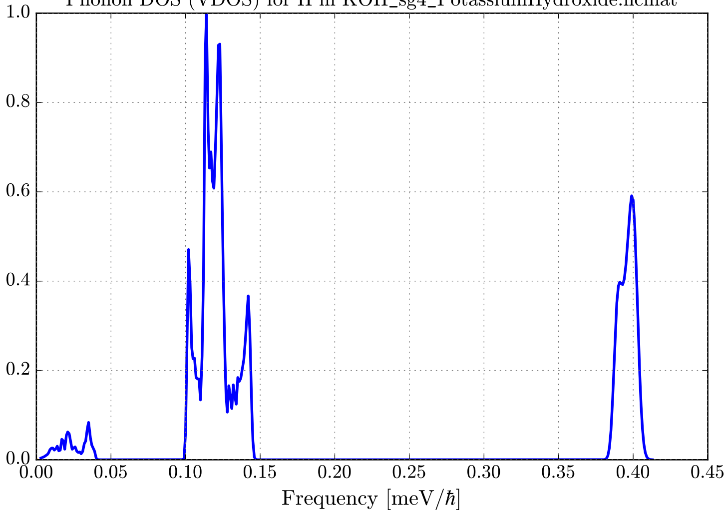
Phonon DOS (VDOS) for H in KOH_sg4_PotassiumHydroxide.ncmat
