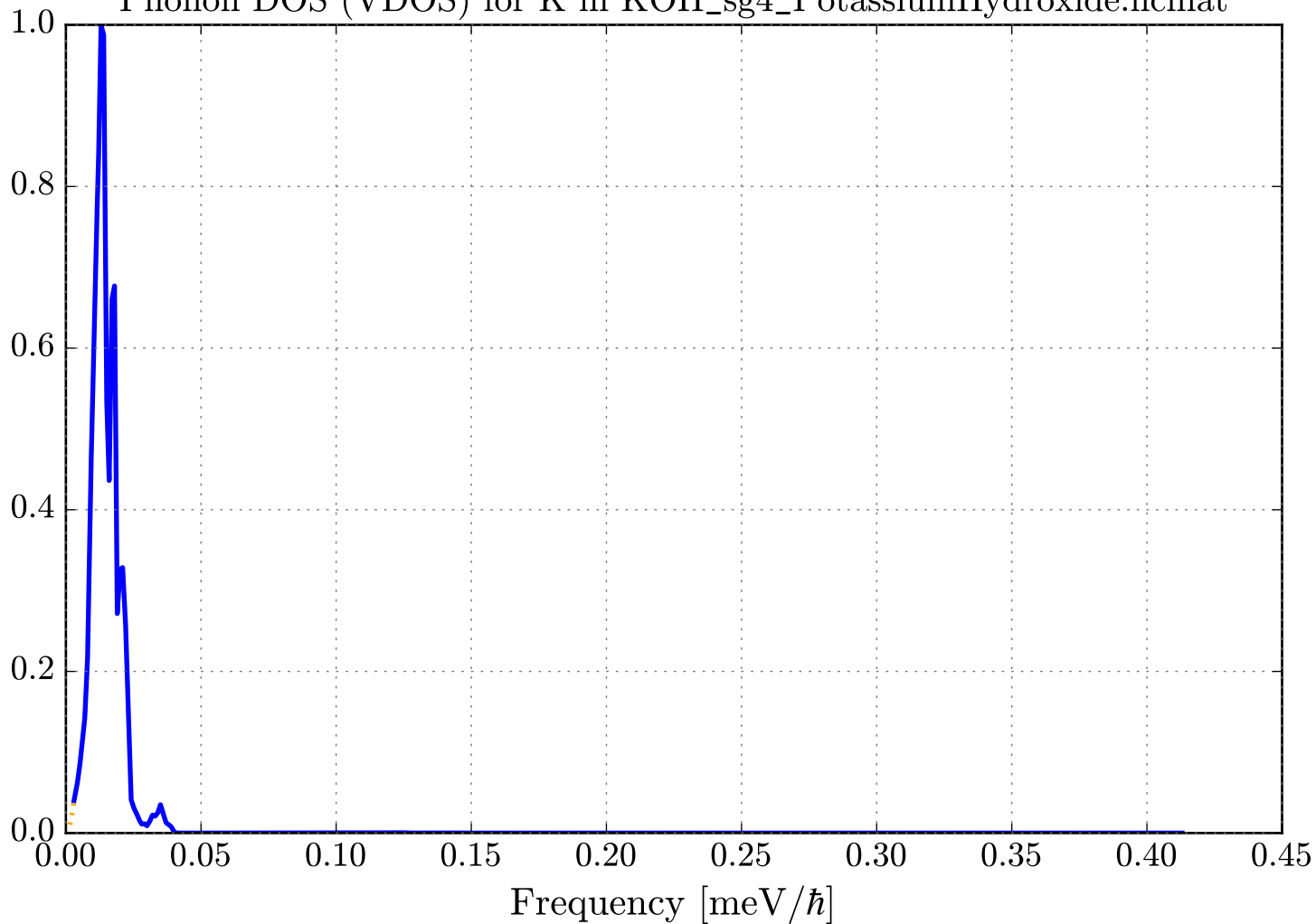
Phonon DOS (VDOS) for K in KOH_sg4_PotassiumHydroxide.ncmat
