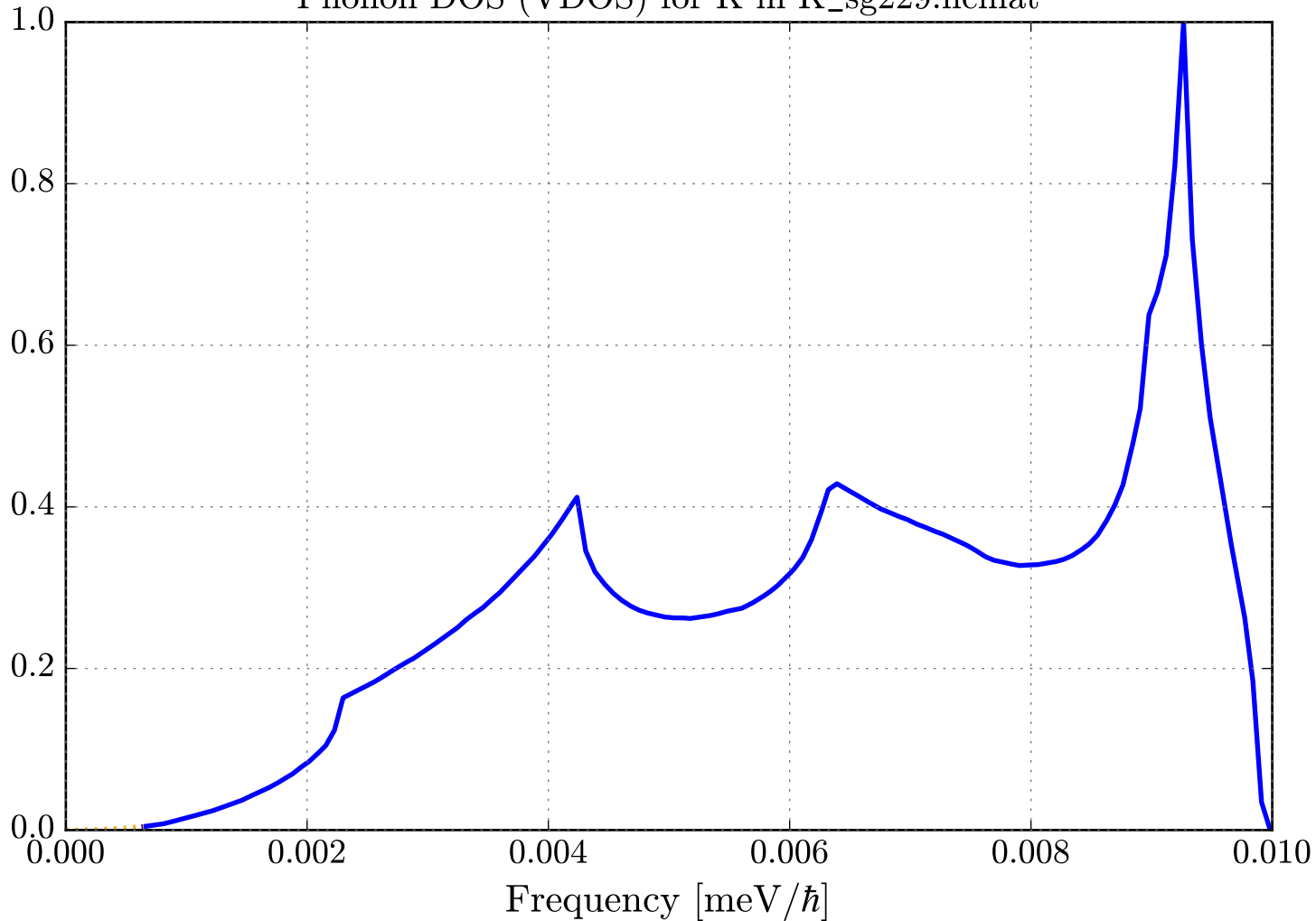
Phonon DOS (VDOS) for K in K_sg229.ncmat
