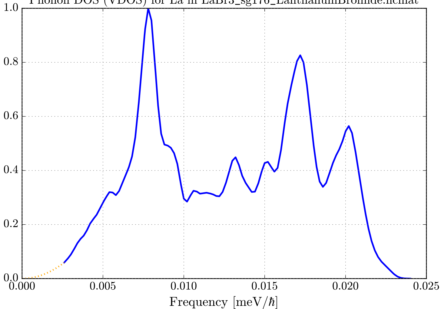
Phonon DOS (VDOS) for La in LaBr3_sg176_LanthanumBromide.ncmat
