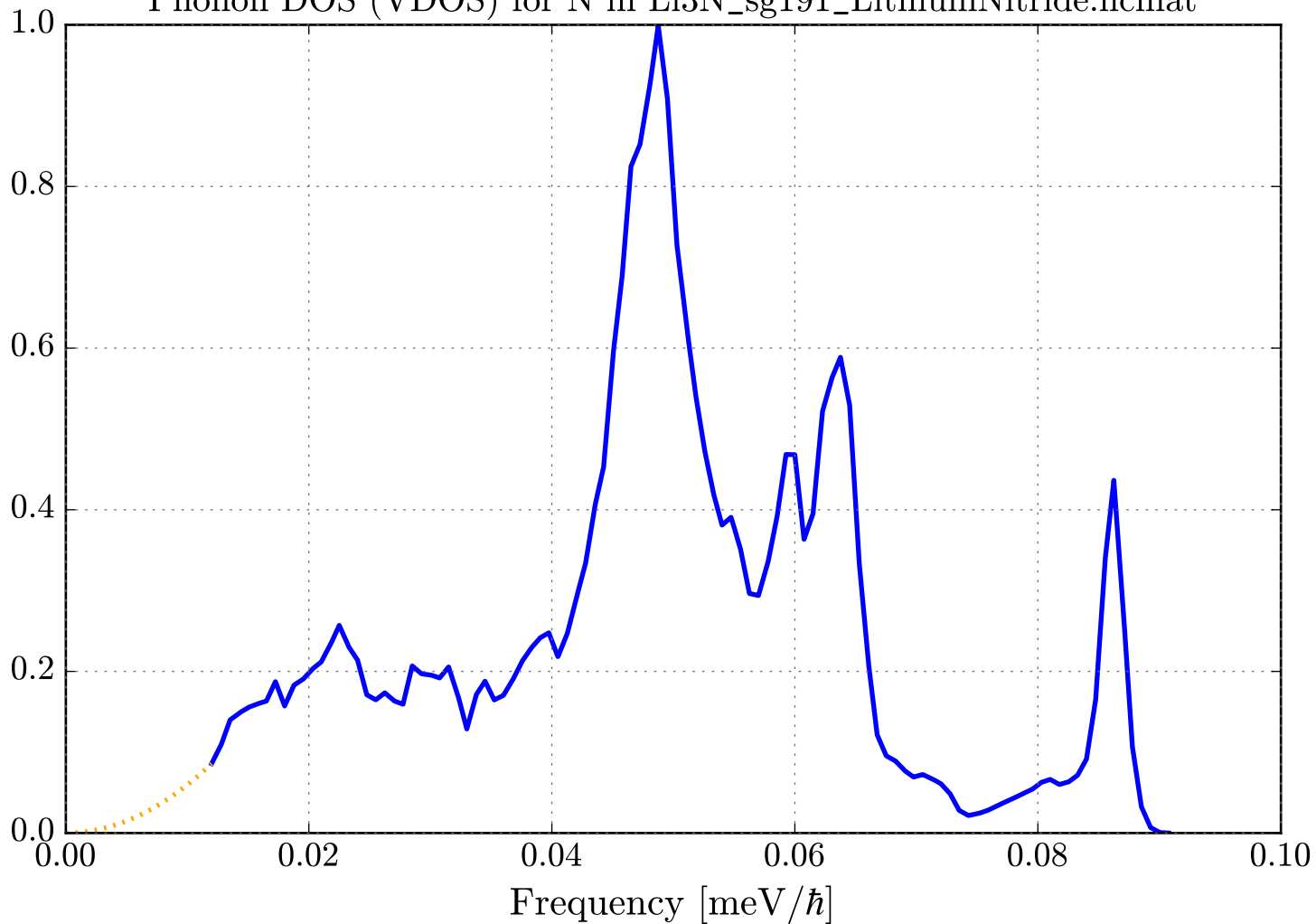
Phonon DOS (VDOS) for N in Li3N_sg191_LithiumNitride.ncmat
