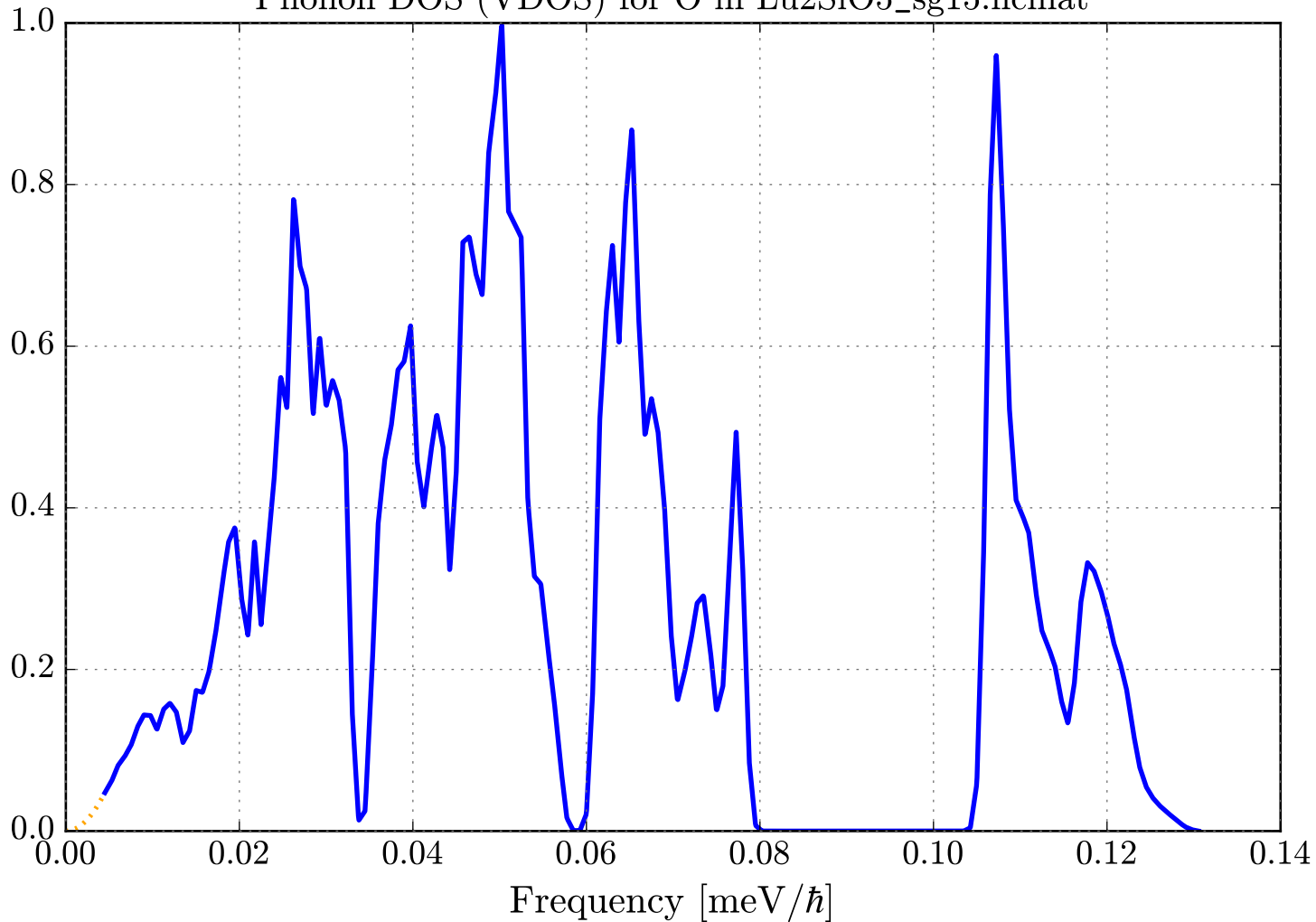
Phonon DOS (VDOS) for O in Lu2SiO5_sg15.ncmat
