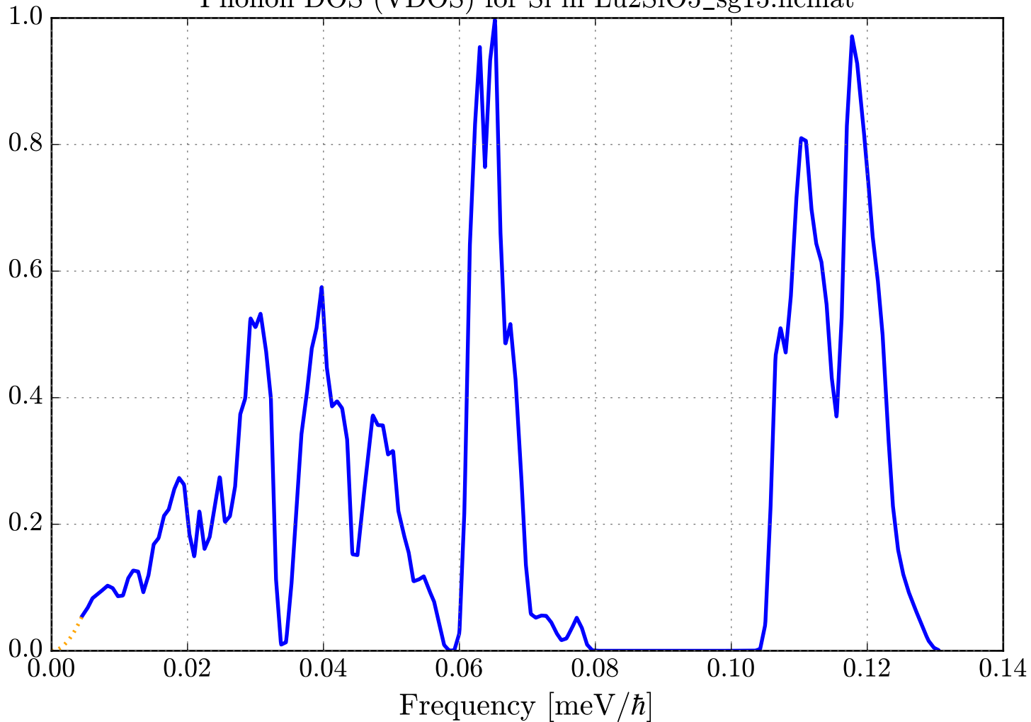
Phonon DOS (VDOS) for Si in Lu 2 SiO 5 _sg15.ncmat
