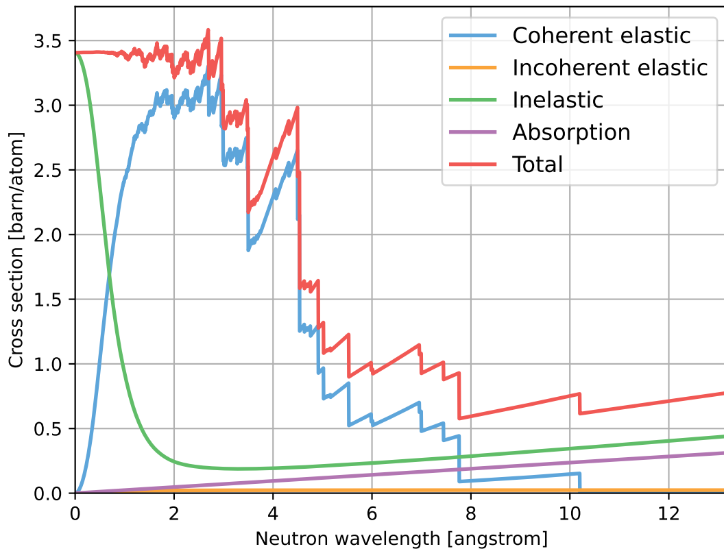
Mg2SiO4_sg62_MagnesiumSilicate.ncmat [dcutoff=0.2]
