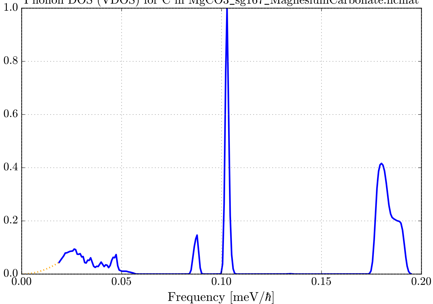
Phonon DOS (VDOS) for C in MgCO3_sg167_MagnesiumCarbonate.ncmat
