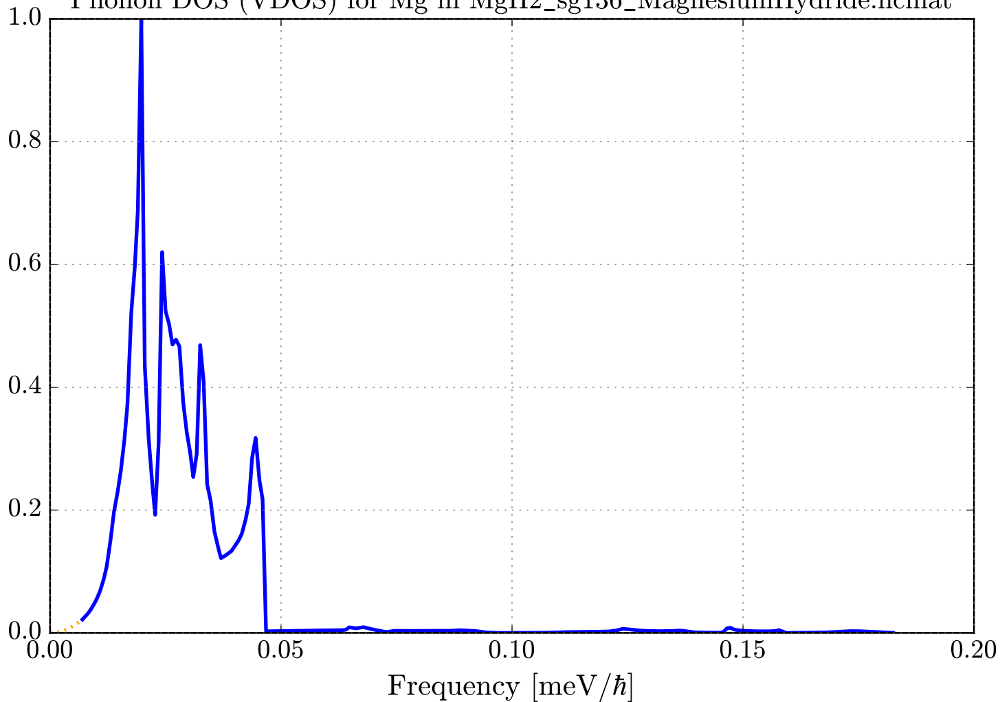
Phonon DOS (VDOS) for Mg in MgH2_sg136_MagnesiumHydride.ncmat
