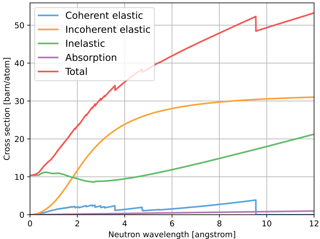
MgO2H2_sg164_MagnesiumHydroxide.ncmat
